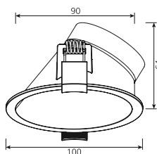
ASYMMETRICAL TRIM Ø95
